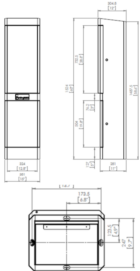
MOUNTING HOLES
