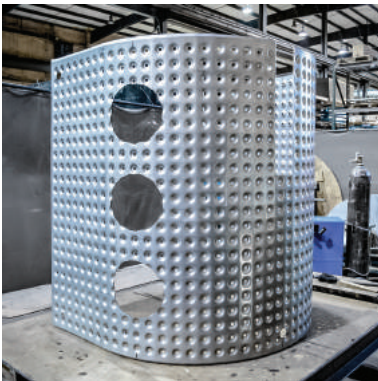
Heat Transfer Dimple Jacket Fabrication
