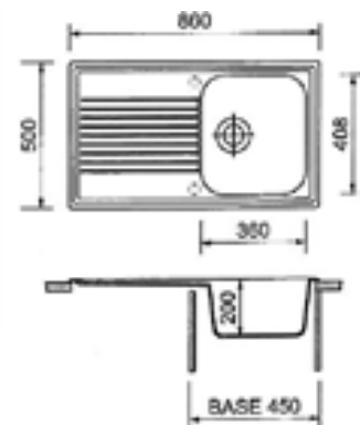
LAVELLO 86 x 50 - LV/1 - 1 vasca ATLANTIC
