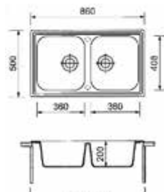
LAVELLO 86 x 50 - LV/2 - 2 vasche ATLANTIC
