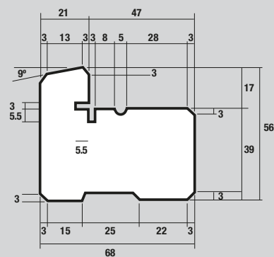
DF-02 56mm x 68mm Head/Jamb
