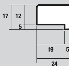
OAK DFC 17mm x 24mm Cill Adaptor
