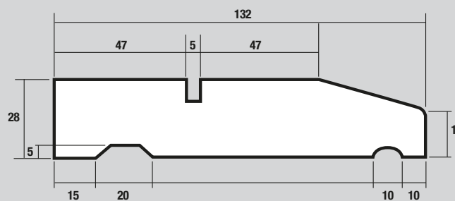
OAK DFC 28mm x 132mm Cill
