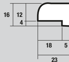
CA-01 16mm x 23mm Cill Adaptor
