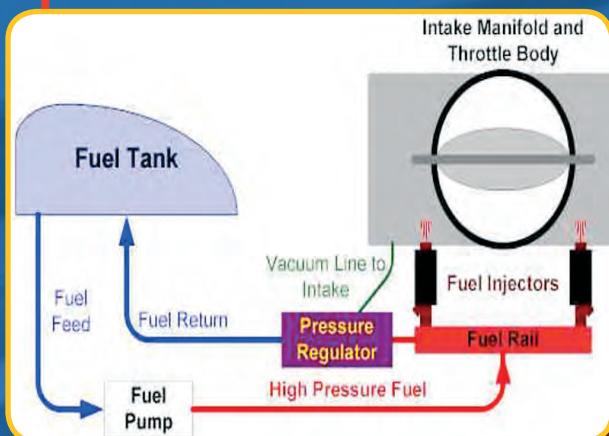
Typical Fuel / Air Intake System
