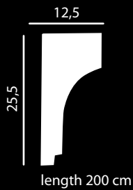
EAVE CORNICE BF9055
