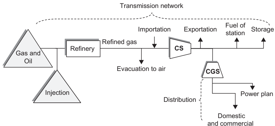
Figure 19.2 The process of transportation during the natural gas network.
