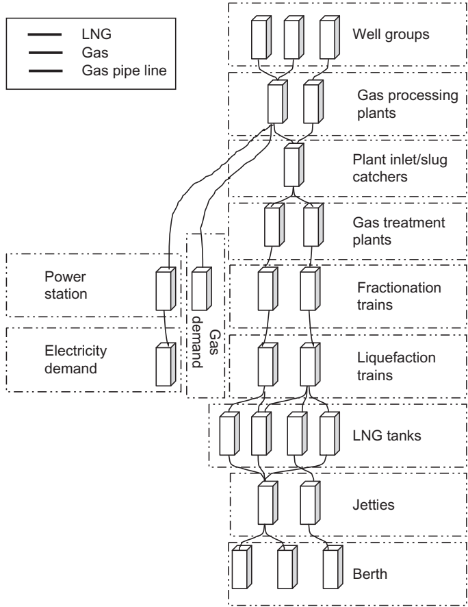
Figure 21.2 The structure of a loading port [9].
