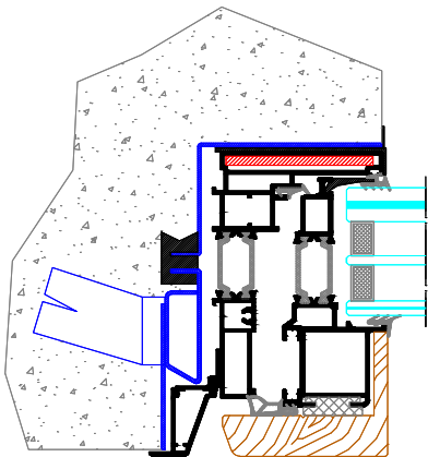
ALLUMINIO RASOMURO ALLUMINIUM FLUSH-WALL WALL PANEL INTERNAL ALUMINIUM IKONA / IKONA WOOD
