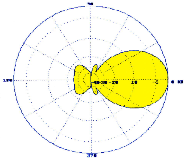
E Plane Plot
