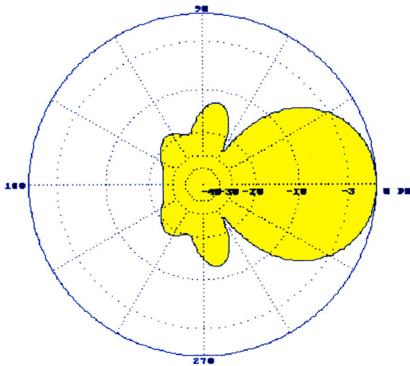
H Plane Plot
