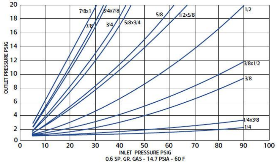
Relief Curves
