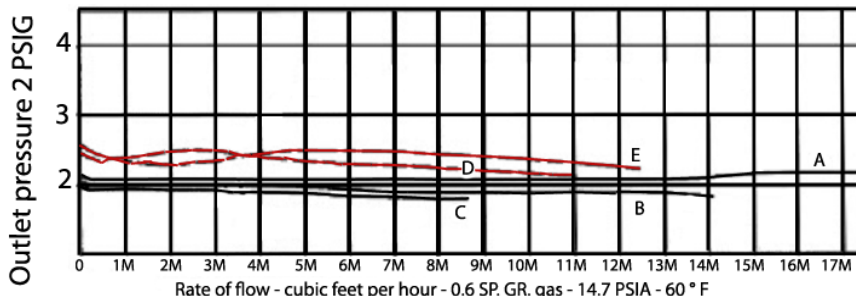
Relief Monitor Curves
