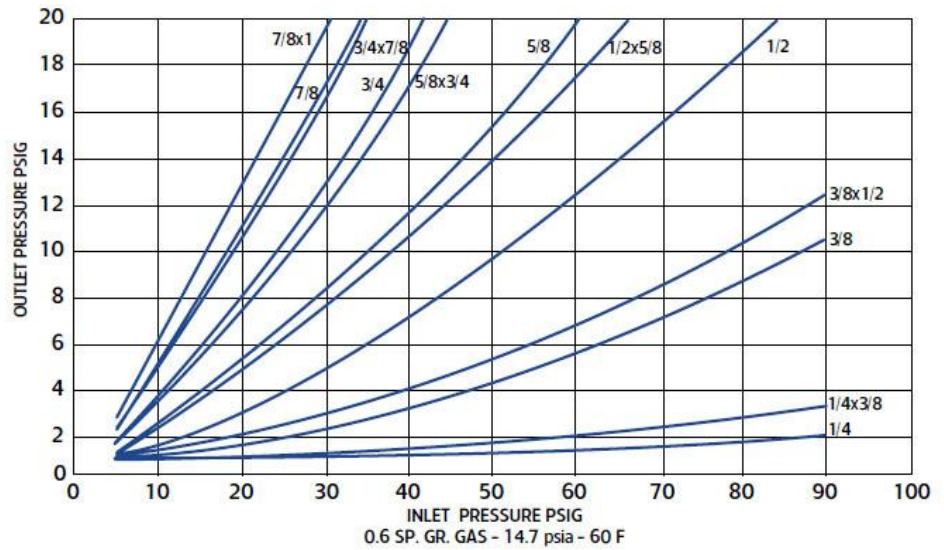
Relief Curves
