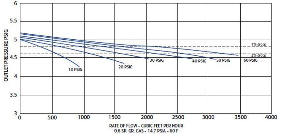
Performance Curves
