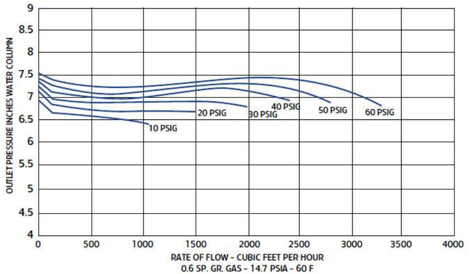
Performance Curves
