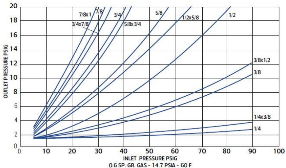
Relief Curves
