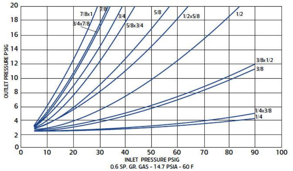
Relief Curves
