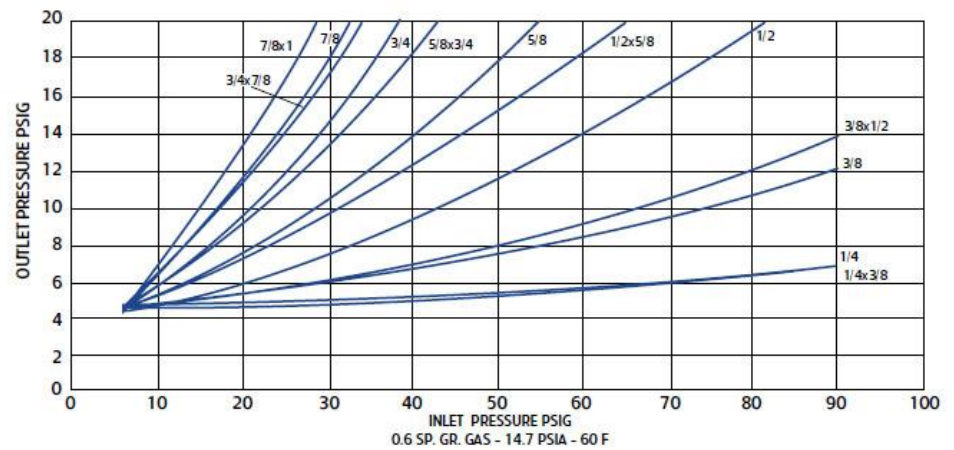
Relief Curves
