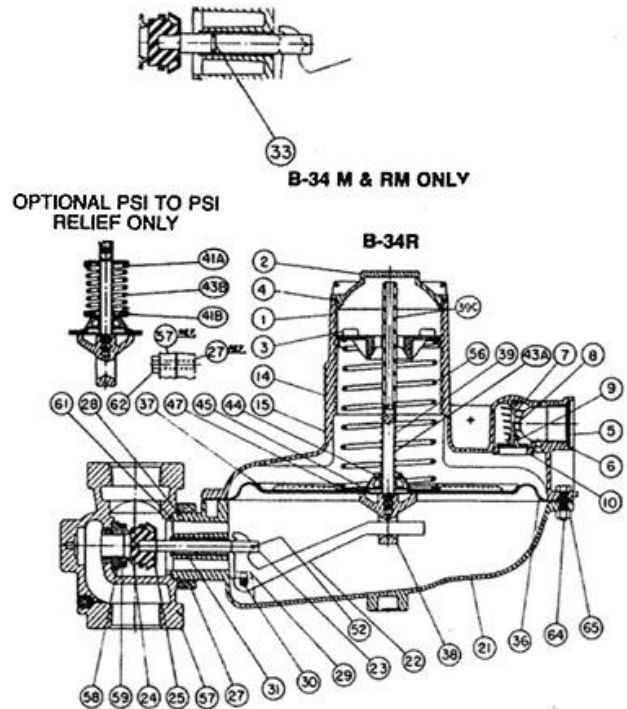
B34R Reference Schematics
