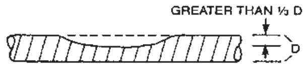
Figure: 5-2 – Repair Necessary. Significant Damage to the Tubing Due to Impact or Crushing
