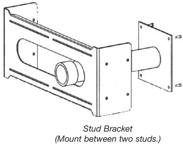
Figure: 4-12 Meter Mounting Accessories
