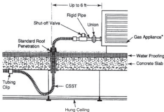
Figure: 4-16 Short (1-6 foot) outdoor connection to roof mounted equipment
