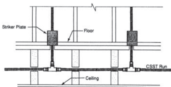
Figure: 4-4 Multiple outlets along main tubing run
