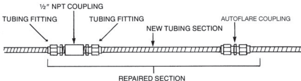
Figure: 5-4 – Repair of Damaged Tubing with a New Section of Tubing and a joint splice or an CounterStrike AutoFlare Coupling
