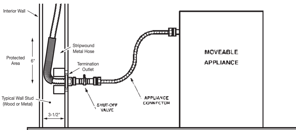
Figure: 4-15 Stainless Steel Gas Connector Connection to a Movable Gas Appliance
