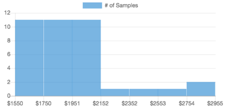
Rent Distribution
