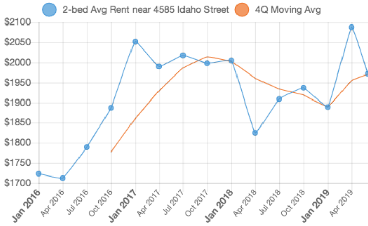
Summary Statistics
