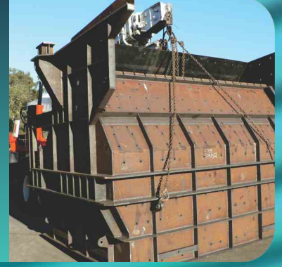
HOPPERS & CHUTES
