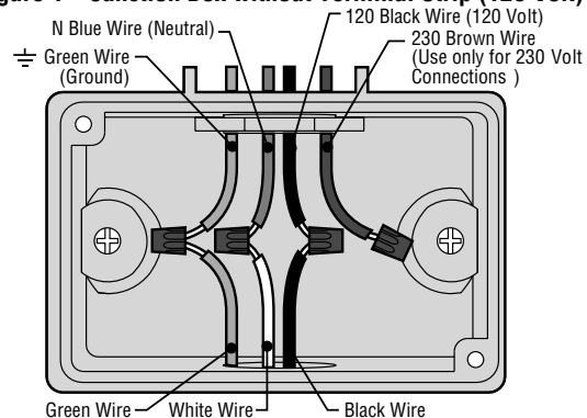
Figure 1 – Junction Box without Terminal Strip (120 Volt)
