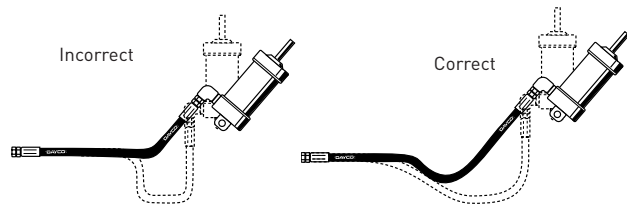
FIGURE 3 — MOTION ABSORPTION
