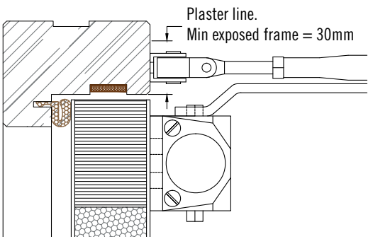
Overhead Closer detail timber frame
