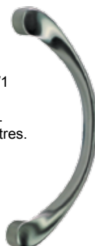
Flessa SC,CP 278mm length. 100mm projection. 247mm hole centres.
