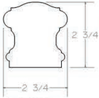
R7700
