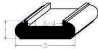
Shoerail 3"W x 1"H (1 3/4" Plow) - R6006OAK - R6006MAPLE
