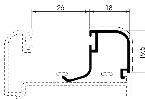
9628/26T peso: Kg./mt. 0.256 sup. in vista: mm. 30
