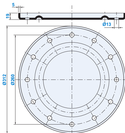
Coperchio 12 fori Couvercle 12 trous
