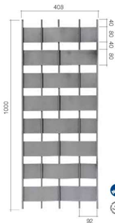
Art. GD303/1 \square 16 x 8 mm L 408 mm H 1000 mm
