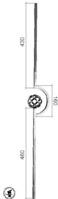
Art. 1090/1 \varnothing 12 mm L 115 mm H 1000 mm
