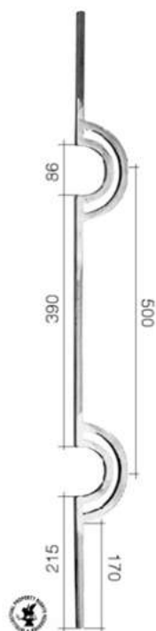
Art. 1090/4 \varnothing 12 mm L 90 mm H 1000 mm
