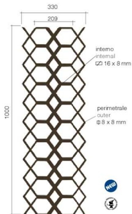
Art. GD299/2 \Phi 8 x 8 mm + \square 16 x 8 mm L 330 mm H 1000 mm
