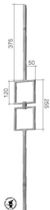
Art. GD182/1 \varnothing 14 mm L 115 mm H 1000 mm
