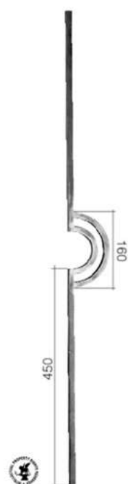
Art. 1090/3 \varnothing 12 mm L 90 mm H 1000 mm
