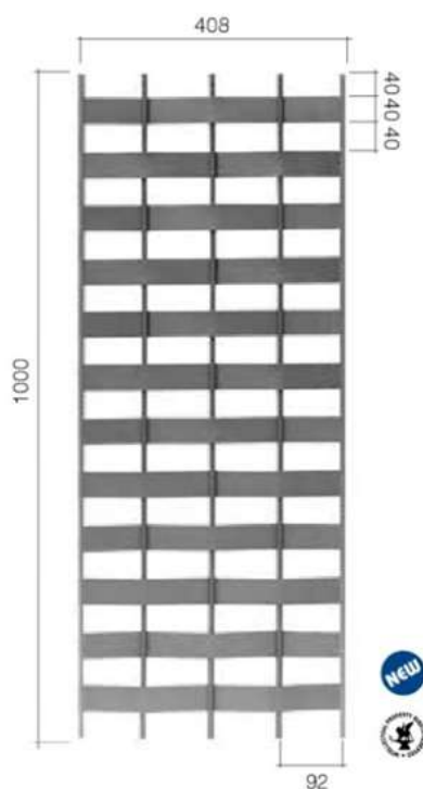
Art. GD303/2 \square 16 x 8 mm L 408 mm H 1000 mm
