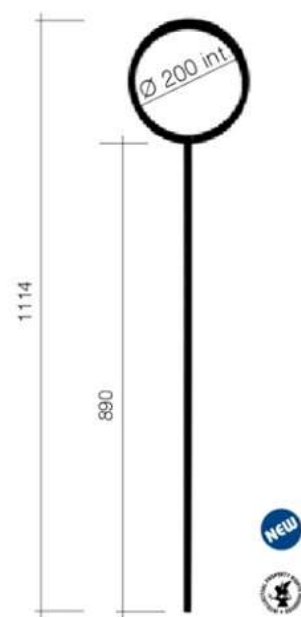
Art. GD296/2 \Phi 12 x 12 mm L \Phi 224 mm H 1114 mm
