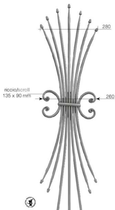
Art. GD255/1 Ø 12 mm L 280 mm H 1000 mm
