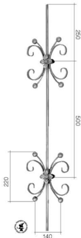
Art. 1061/2 Ø 12 mm H 1000 mm L 205 mm
