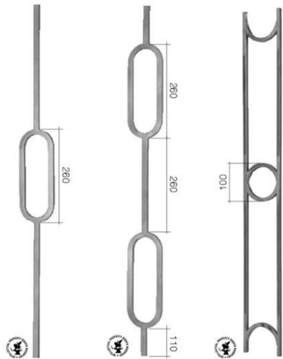
Art. GD29/1 Ø 14 mm L 100 mm H 1000 mm
