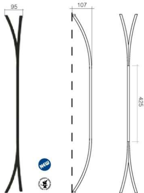
Art. GD290/1 \varnothing 12 x 12 mm H 1000 mm
