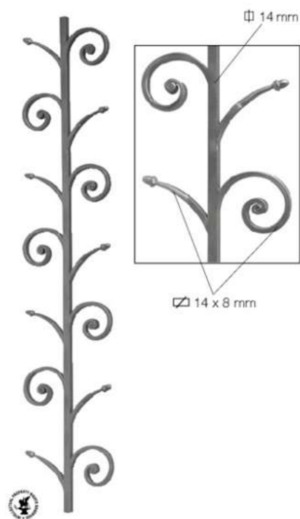
Art. GD176/1 \varnothing 14 mm L 200 mm H 1000 mm
