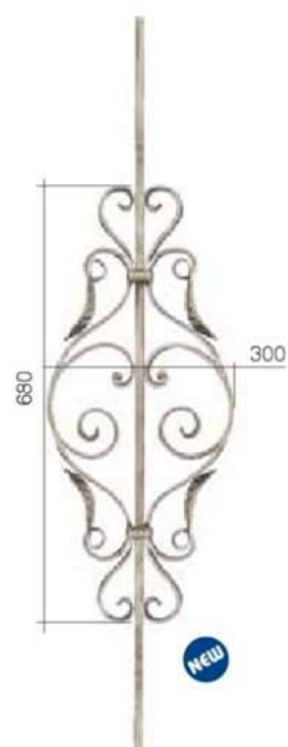
Art. GD27/1 Ø 14 mm L 300 mm H 1000 mm
