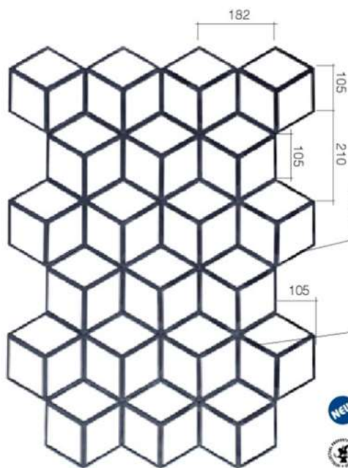
Art. GD287/1 \sphericalangle 12 \times 6 \text{ mm} + \Phi 12 \text{ mm} H 1000 mm L 728 mm
