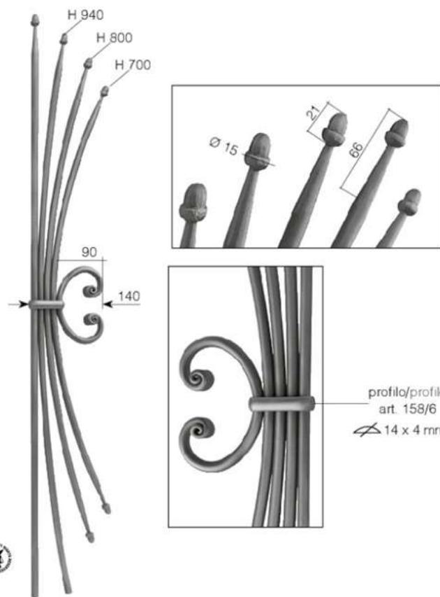
Art. GD255/2 Ø 12 mm L 150 mm H 1000 mm
