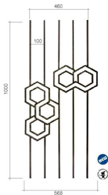
Art. GD301/3 \Phi 12 x 12 mm L 568 mm H 1000 mm
