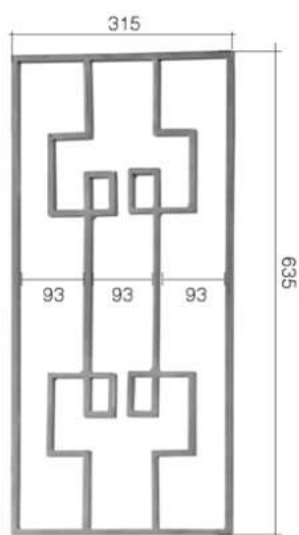
Art. GD202/4 □ 14 x 8 mm L 315 mm H 635 mm
