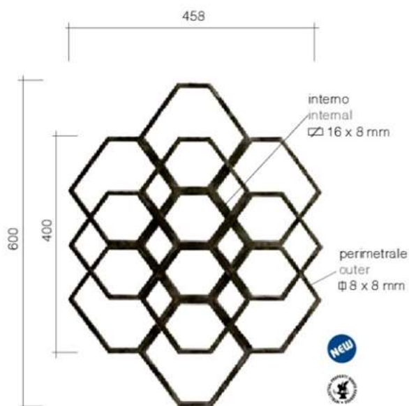
Art. GD299/4 \Phi 8 x 8 mm + \square 16 x 8 mm L 458 mm H 600 mm
