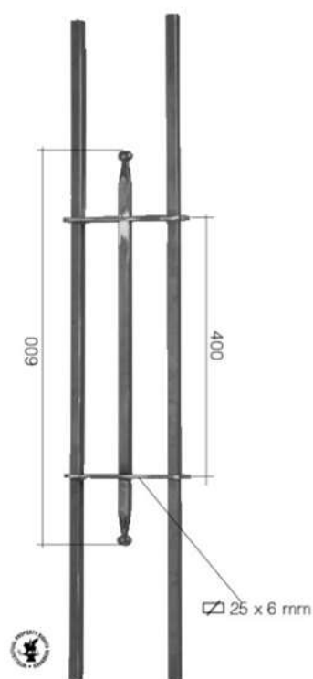
Art. GD66/1 \Phi 12 x 12 mm L 125 mm H 1000 mm
