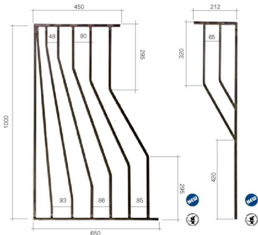
Art. GD212/2 \Phi 12 x 12 mm L 650 mm H 1000 mm
