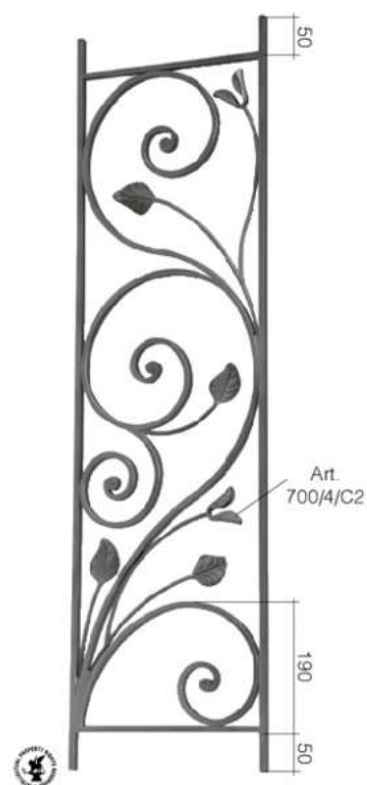
Art. GD223/1 ▧ 14 x 8 mm H 1000 mm L 275 mm
