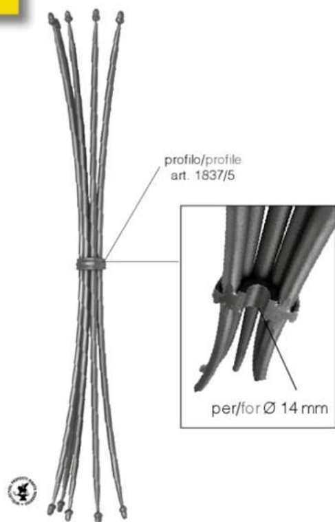
Art. GD253/1 Ø 12 mm L 150 mm H 870 mm
