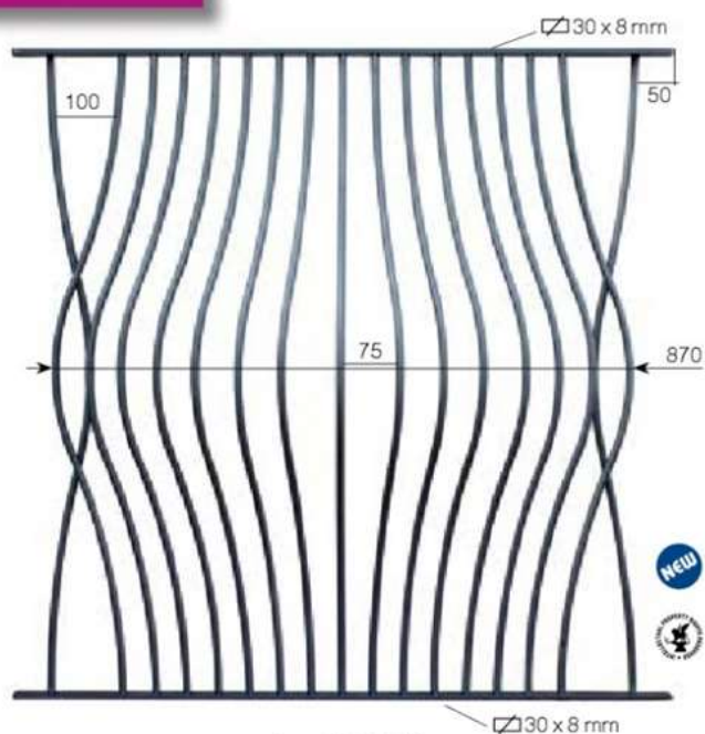
Art. GD288/1 Ø 12 mm L1000 mm H 1000 mm
