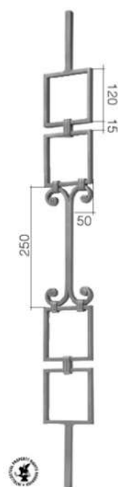
Art. GD184/2 \varnothing 14 mm L 115 mm H 1000 mm
