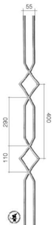
Art. GD19/2 □ 14 x 8 mm L 100 mm H 1000 mm
