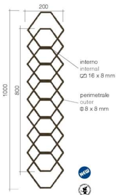
Art. GD299/3 \Phi 8 x 8 mm + \square 16 x 8 mm L 200 mm H 1000 mm
