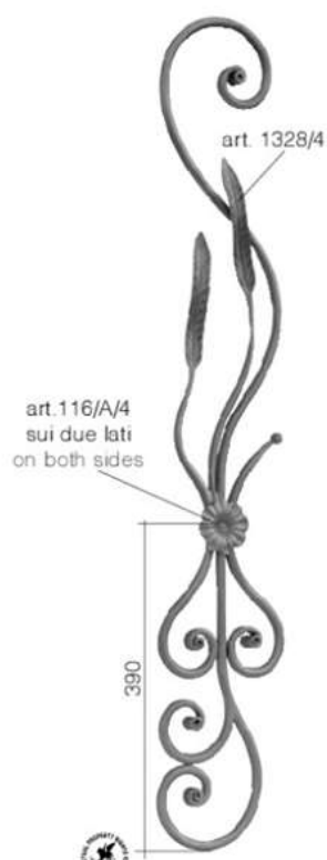
Art. GD170/2 Ø 12 mm L 170 mm H 1000 mm
