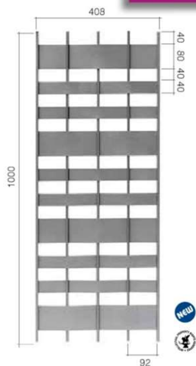
Art. GD303/3 \square 16 x 8 mm L 408 mm H 1000 mm
