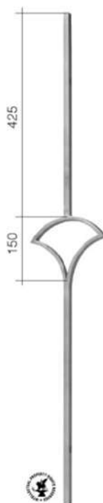
Art. GD186/1 \varnothing 14 mm L 170 mm H 1000 mm
