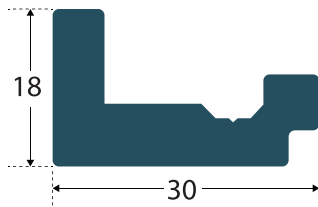
WideBoard Starter Trim
