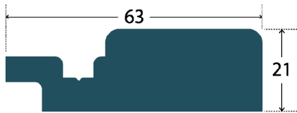
Original/WeatherLap Starter Trim
