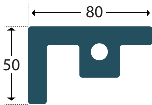
Eco Cladding Internal/External Sleek Corner Trim & Expansion Joint
