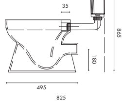
P TRAP
