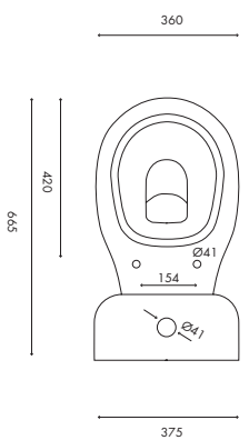
S TRAP
