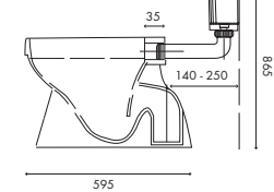
S TRAP
