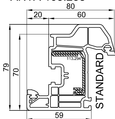
ANTA 103.238
