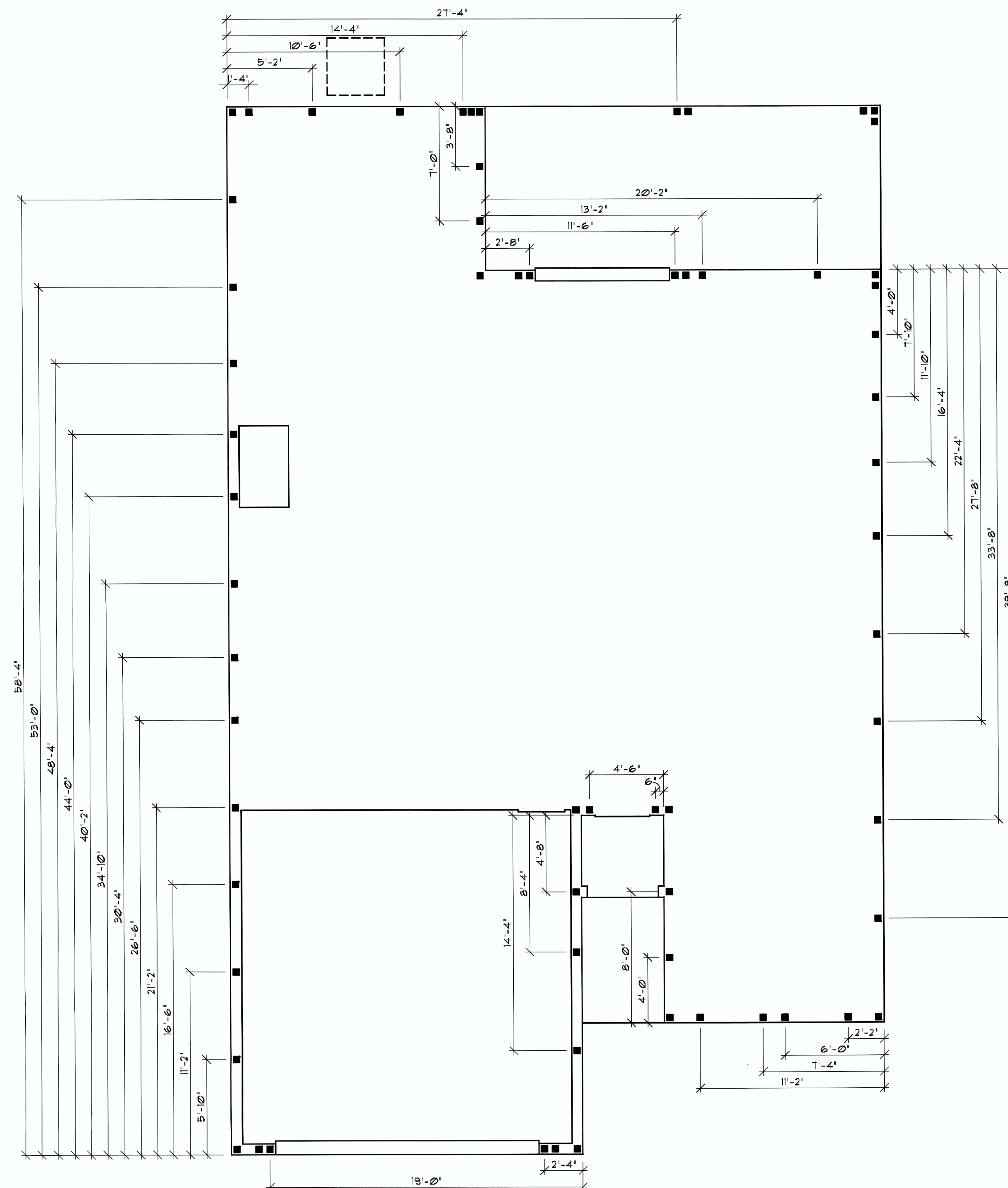
DOWEL PLAN
