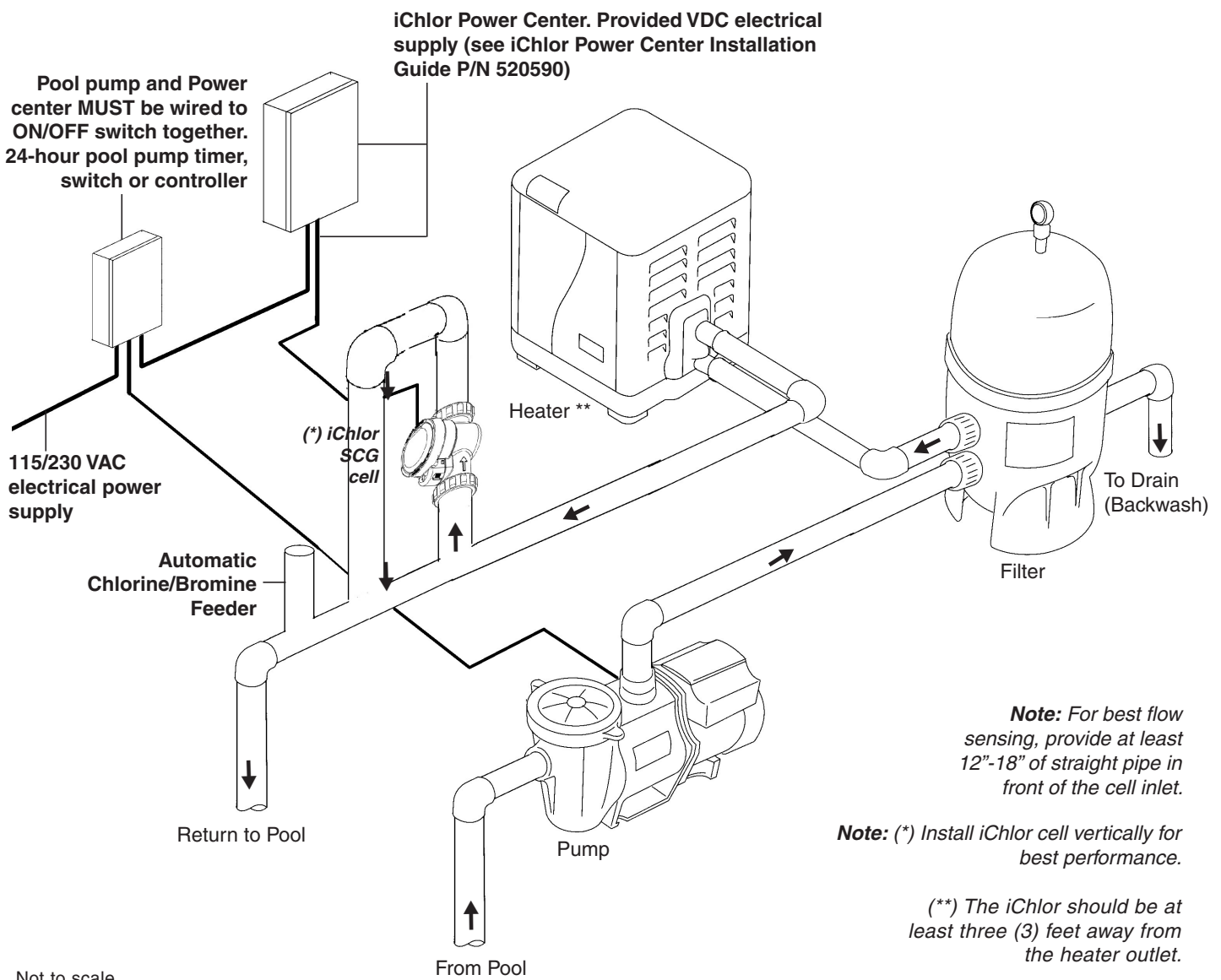
iChlor System Schematic Diagram
