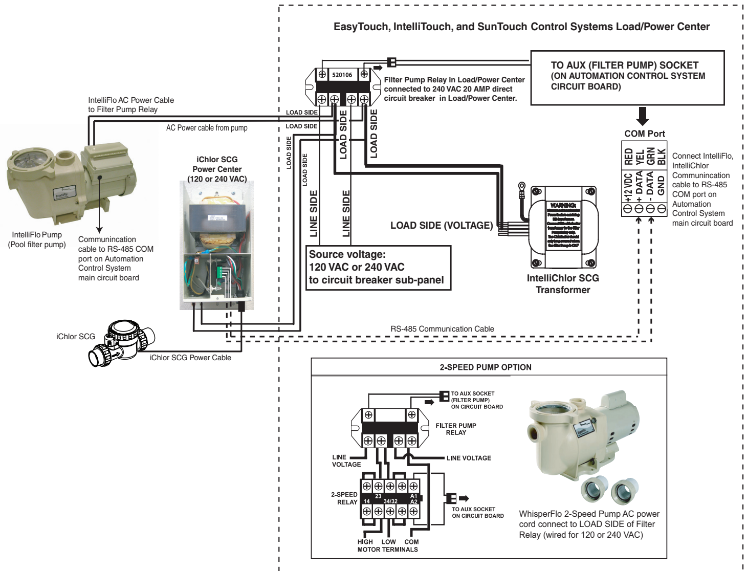
Wiring iChlor™ SCG AC Power Cord to Automation Control System Filter Pump Relay
