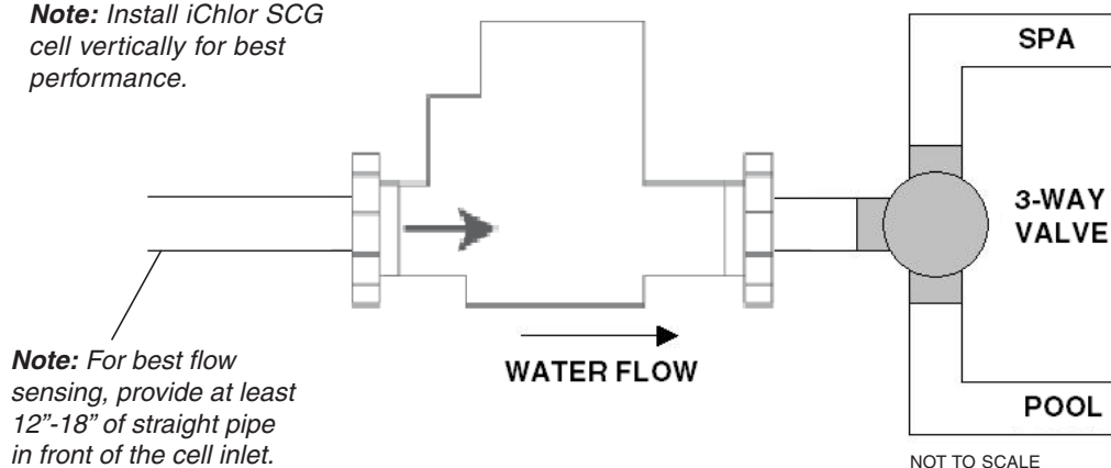
iChlor SCG System Plumbing Diagram
