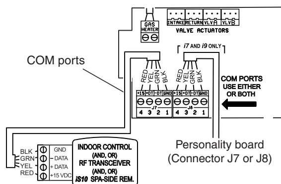
IntelliTouch Control System Personality Circuit Board
