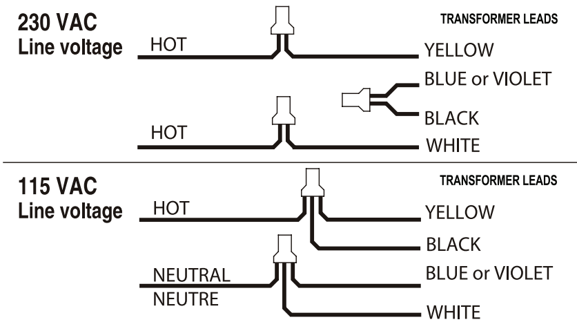
iChlor Power Center 230 and 115 VAC Transformer Wiring
