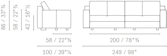
Square cushions
