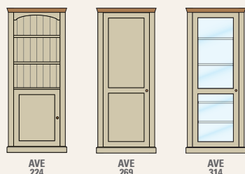
72" x 30" x 15" Lower Door AVE224 H 1830 x W 765 x D 445 72" x 30" x 15" Full Panelled Door AVE269 H 1830 x W 765 x D 445 72" x 30" x 15" Full Glazed Door AVE314 H 1830 x W 765 x D 445
