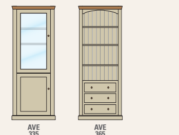
78" x 30" x 15" Semi Glazed Doors - 2 doors AVE335 H 1980 x W 765 x D 445 78" x 30" x 15" Lower Drawers AVE365 H 1980 x W 765 x D 445
