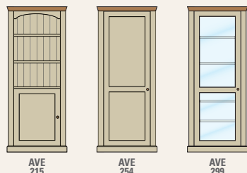
72" x 30" x 12" Lower Door AVE215 H 1830 x W 765 x D 360 72" x 30" x 12" Full Panelled Door AVE254 H 1830 x W 765 x D 360 72" x 30" x 12" Full Glazed Door AVE299 H 1830 x W 765 x D 360
