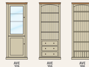
78" x 30" x 12" Semi Glazed Doors - 2 doors AVE329 H 1980 x W 765 x D 360 78" x 30" x 12" Lower Drawers AVE359 H 1980 x W 765 x D 360 78" x 30" x 15" Open Shelved AVE200 H 1980 x W 765 x D 445
