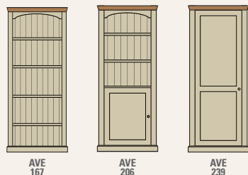
72" x 30" x 9" Open Shelved AVE167 H 1830 x W 765 x D 285 72" x 30" x 9" Lower Door AVE206 H 1830 x W 765 x D 285 72" x 30" x 9" Full Panelled Door AVE239 H 1830 x W 765 x D 285
