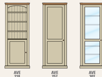
78" x 30" x 12" Lower Door AVE218 H 1980 x W 765 x D 360 78" x 30" x 12" Full Panelled Door AVE257 H 1980 x W 765 x D 360 78" x 30" x 12" Full Glazed Door AVE302 H 1980 x W 765 x D 360
