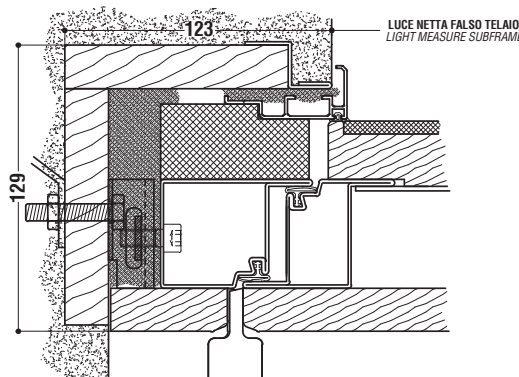
NODO LATERALE / SIDE NODE CERNIERA A VISTA / EXPOSED HINGE
