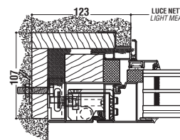
NODO LATERALE E SUPERIORE SIDE AND UPPER NODE CERNIERA A SCOMPARSA / CONCEALED HINGE
