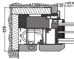
NODO LATERALE E SUPERIORE SIDE AND UPPER NODE CERNIERA A SCOMPARSA / CONCEALED HINGE
