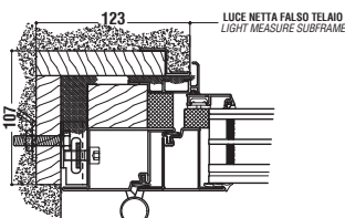
NODO LATERALE E SUPERIORE SIDE AND UPPER NODE CERNIERA A VISTA / EXPOSED HINGE
