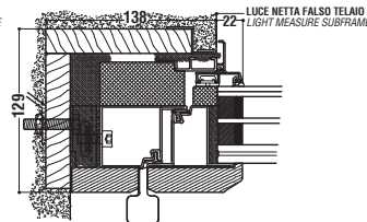
NODO LATERALE E SUPERIORE SIDE AND UPPER NODE CERNIERA A VISTA / EXPOSED HINGE
