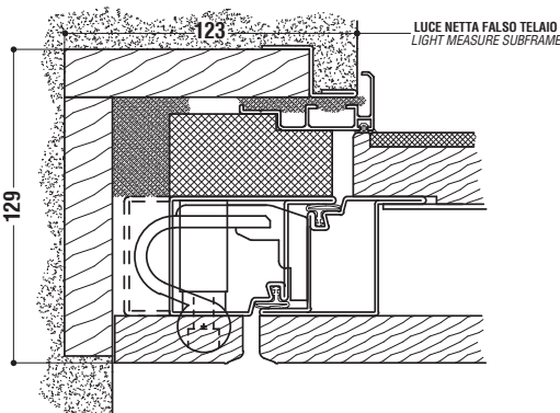
NODO LATERALE / SIDE NODE CERNIERA A SCOMPARSA / CONCEALED HINGE
