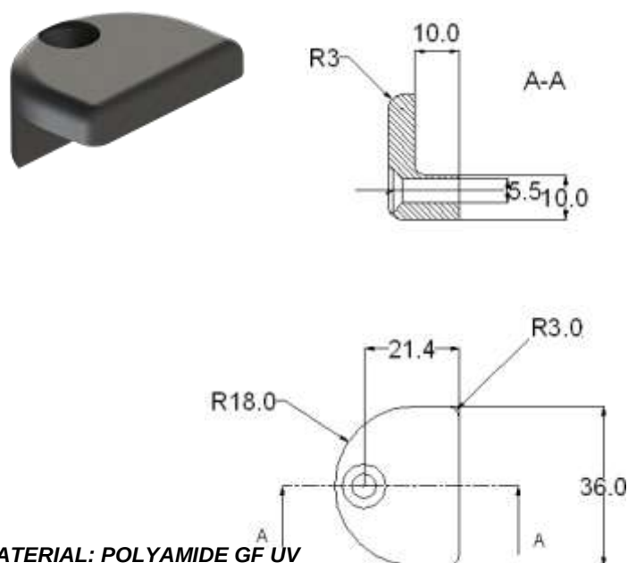
FIXING GLASS BLOCKS CODE 145294
