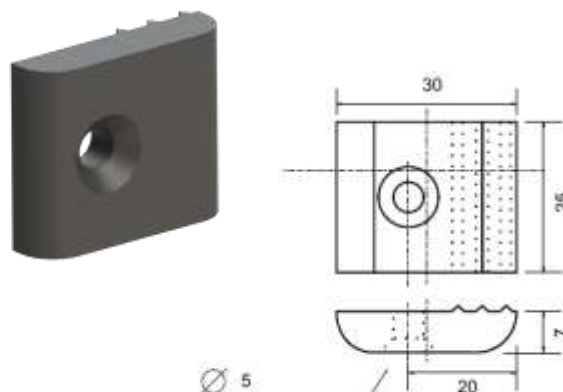
FIXING GLASS BLOCKS CODE 145298
