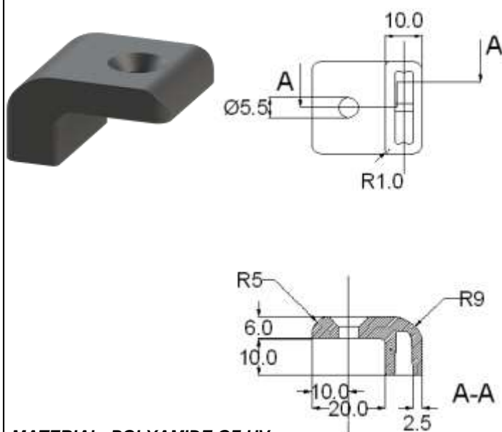
KNOB FOR GENERAL USES CODE 130036
