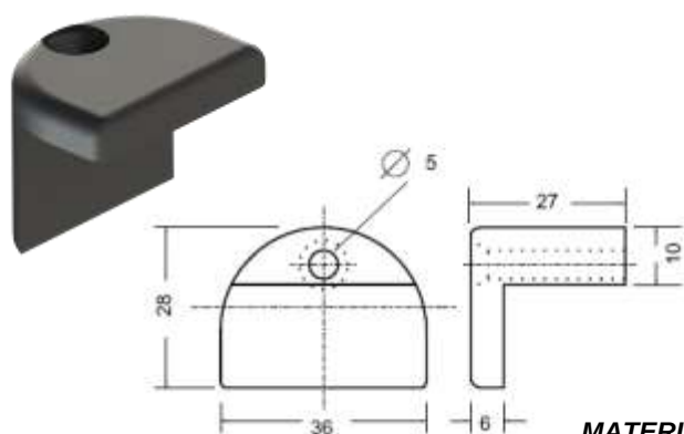
FIXING GLASS BLOCKS CODE 145295
